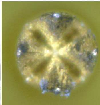
20,000 Insertion Clean every 5,000 insertion BEFORE cleaning
